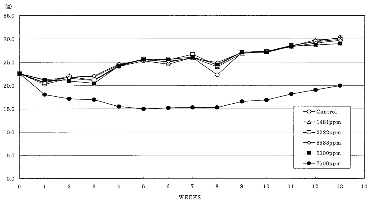
FIGURE 1 BODY WEIGHT CHANGES OF MALE MICE IN THE 13-WEEK FEED STUDY OF 1,4-DICHLORO-2-NITROBENZENE
