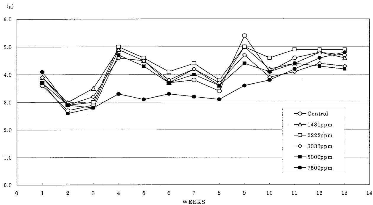
FIGURE 3 FOOD CONSUMPTION CHANGES OF MALE MICE IN THE 13-WEEK FEED STUDY OF 1,4-DICHLORO-2-NITROBENZENE
