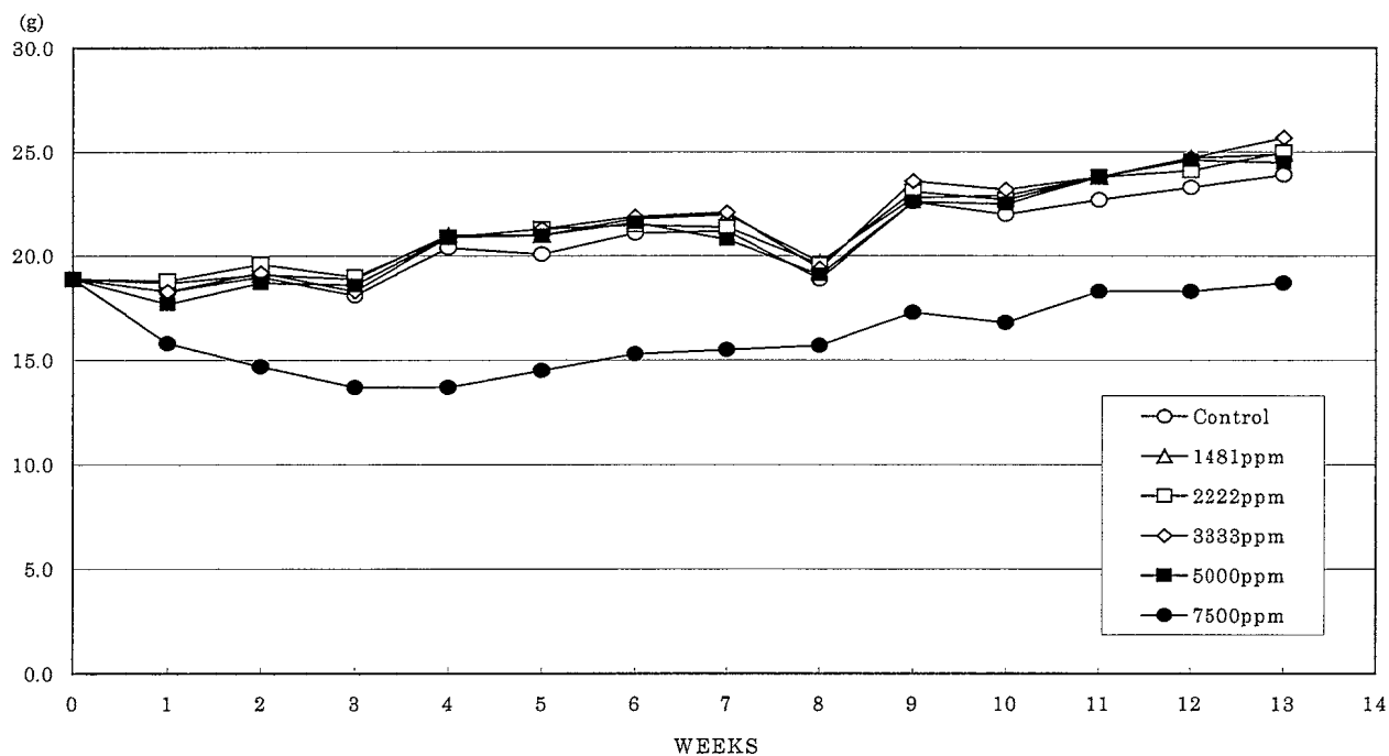
FIGURE 2 BODY WEIGHT CHANGES OF FEMALE MICE IN THE 13-WEEK FEED STUDY OF 1,4-DICHLORO-2-NITROBENZENE
