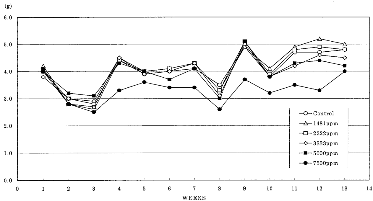
FIGURE 4 FOOD CONSUMPTION CHANGES OF FEMALE MICE IN THE 13-WEEK FEED STUDY OF 1,4-DICHLORO-2-NITROBENZENE
