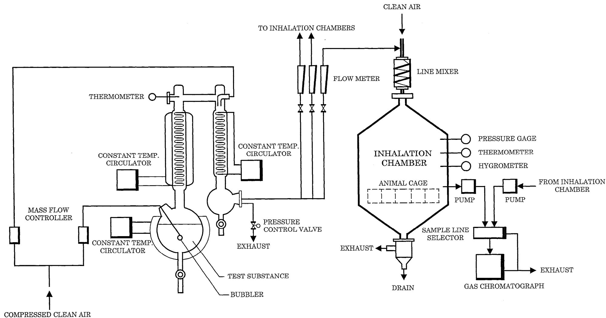
FIGURE 1 1,2-DICHLOROPROPANE VAPOR GENERATION SYSTEM AND INHALATION SYSTEM
