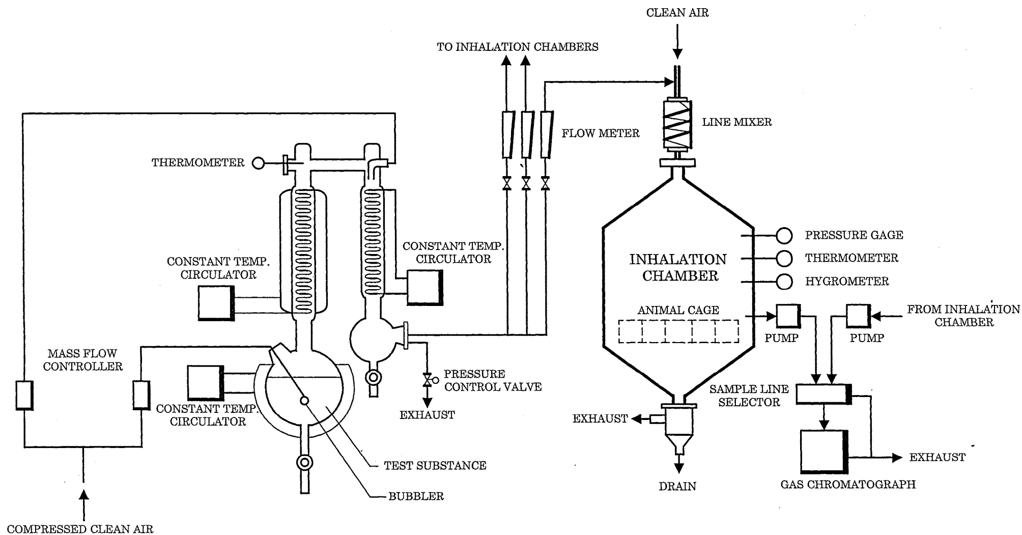
FIGURE 1 2,4-PENTANEDIONE VAPOR GENERATION SYSTEM AND INHALATION SYSTEM
