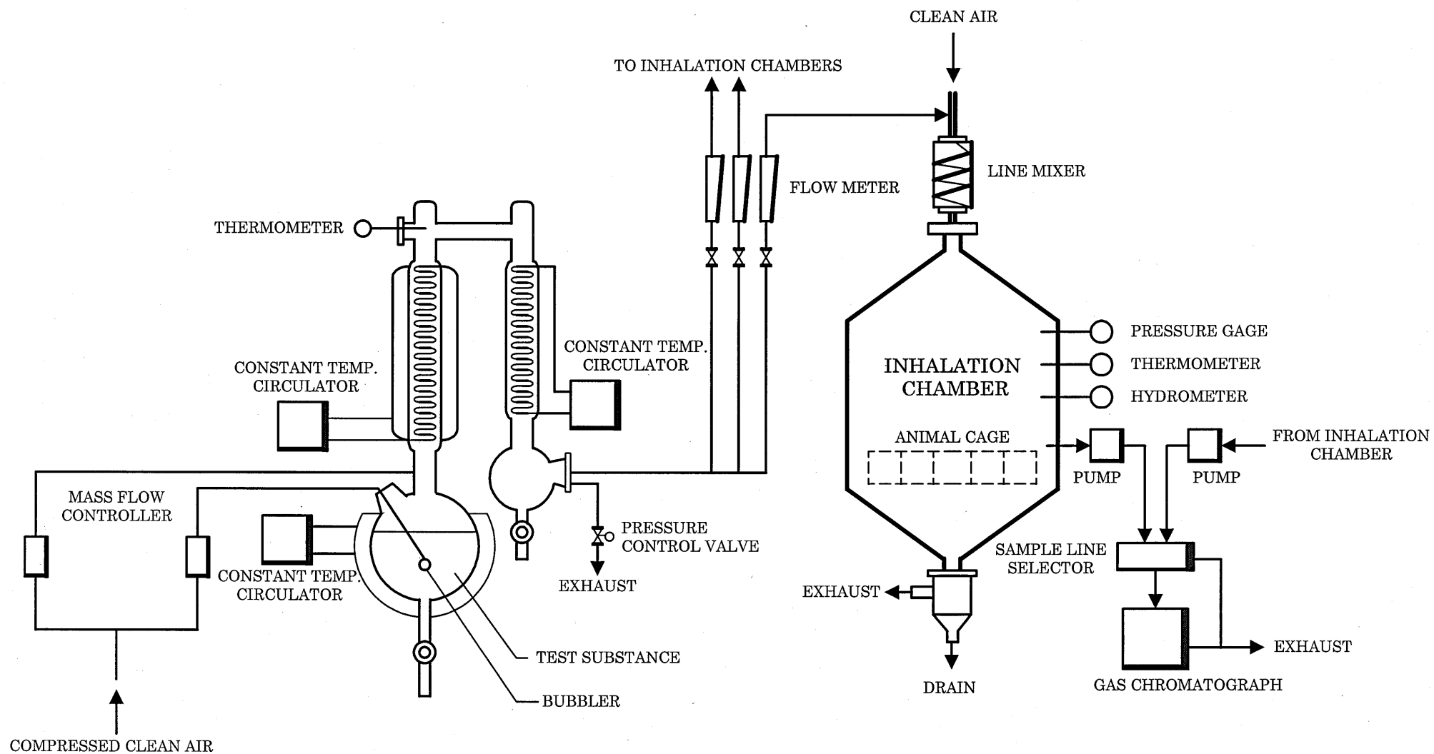
FIGURE 1 ETHYLENE GLYCOL MONOETHYL ETHER ACETATE VAPOR GENERATION SYSTEM AND INHALATION SYSTEM
