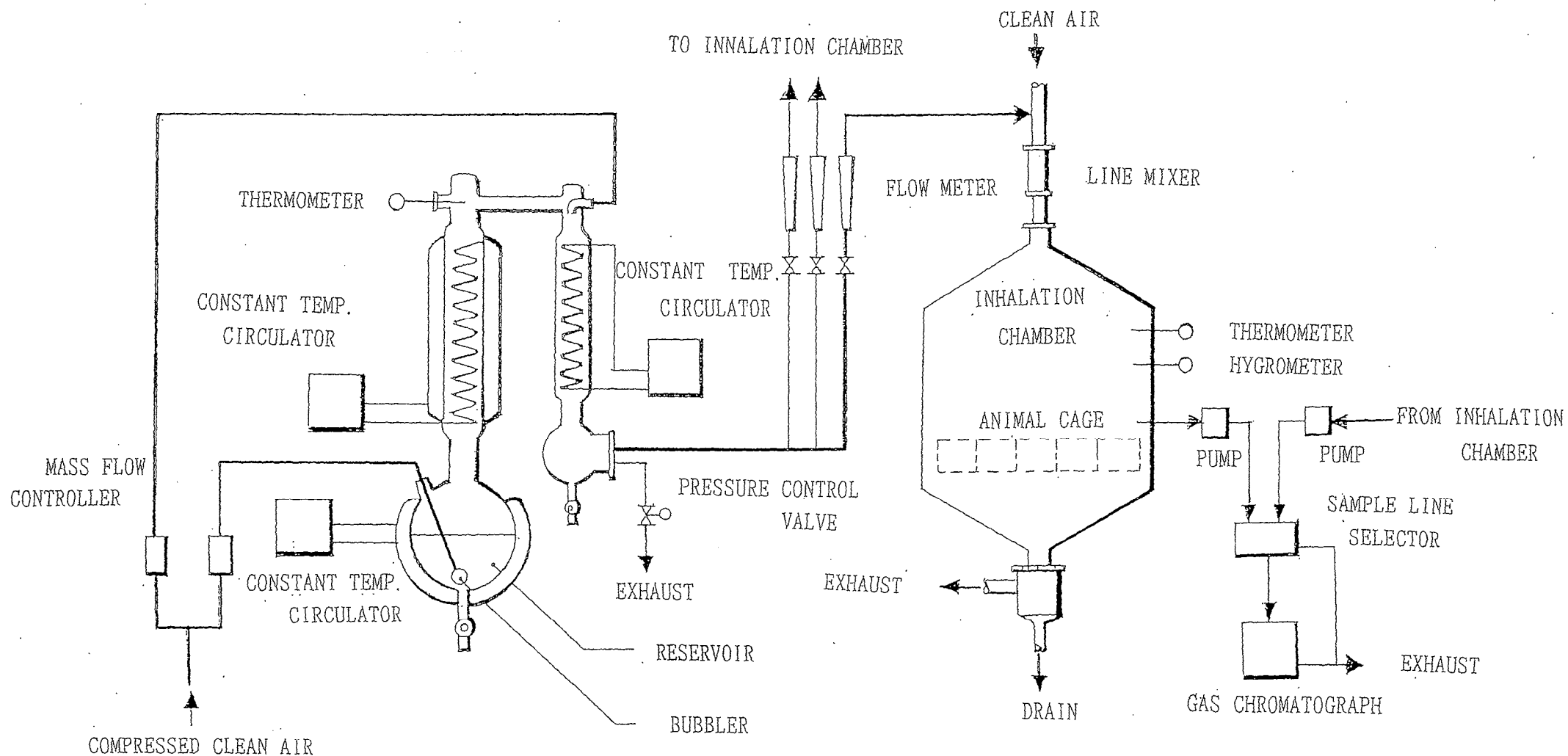
FIGURE 1 1,1,1-TRICHLOROETHANE VAPOR GENERATION SYSTEM AND INHALATION SYSTEM
